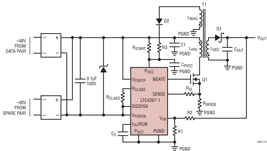
Figure 11. Typical LTC4267-1 Application Circuits
