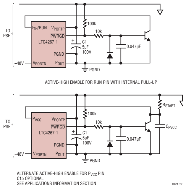
Figure 7. Power Good Interface Examples
