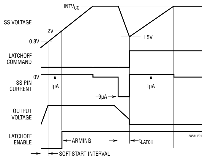
Figure 1. Latchoff Timing Diagram
