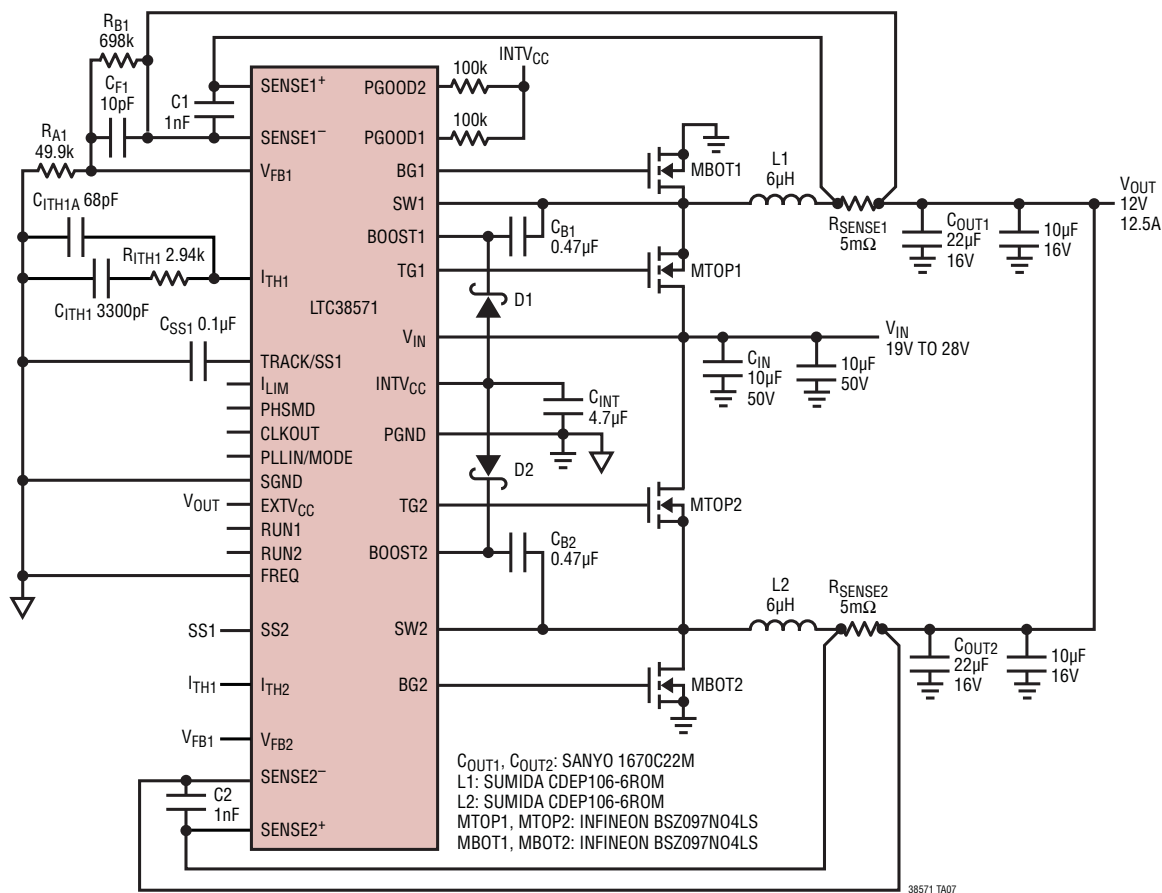
High Efficiency 2-Phase 12V/150W Step-Down Converter
