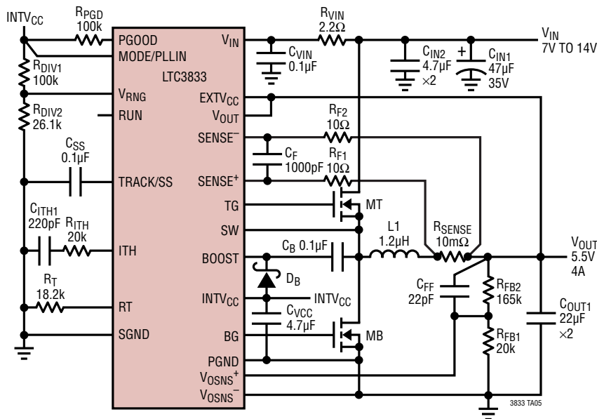
CIN1: KEMET T521X476M035ATE070 CIN2: KEMET T521X476M035ATE070 L1: WURTH 744313120 DB: DIODES, INC. SDM10K45 MT, MB: INFINEON BSC093N04LS
