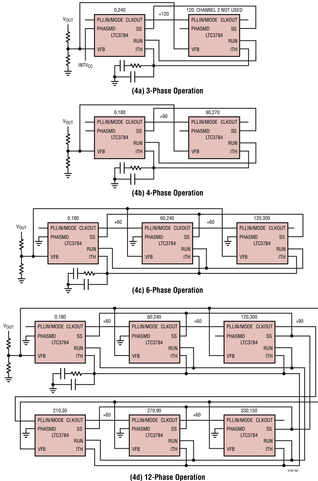
Figure 4. PolyPhase Operation
