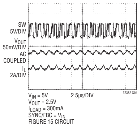
Light Load (Pulse-Skipping Mode)
