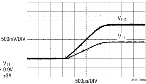
Ratiometric Start-Up
