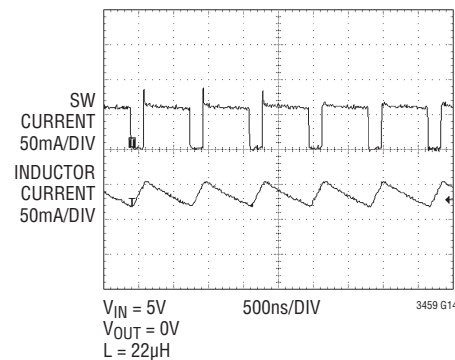
Shorted Output
