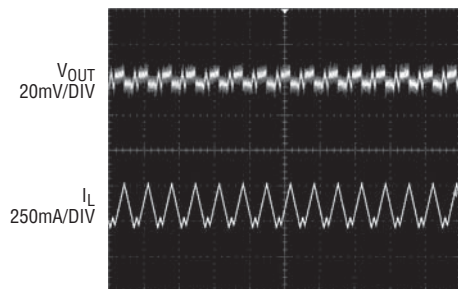
OUT1 Pulse Skipping Mode Operation
