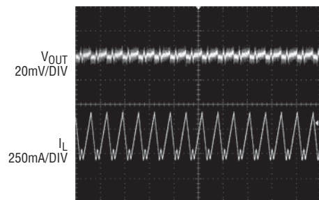
OUT2 Pulse Skipping Mode Operation
