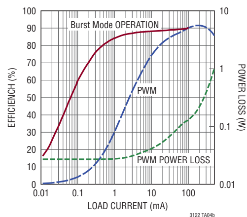
3.3V to 12V, 300kHz Synchronous Boost Converter with Output Disconnect, 500mA
