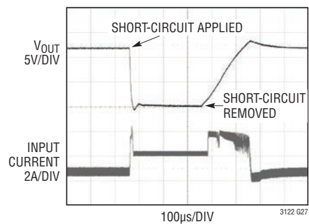
Short-Circuit Response
