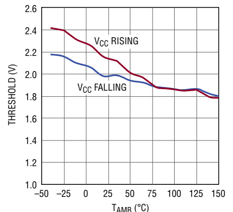
POR Thresholds vs Temperature
