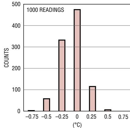
T_{INT} Noise
