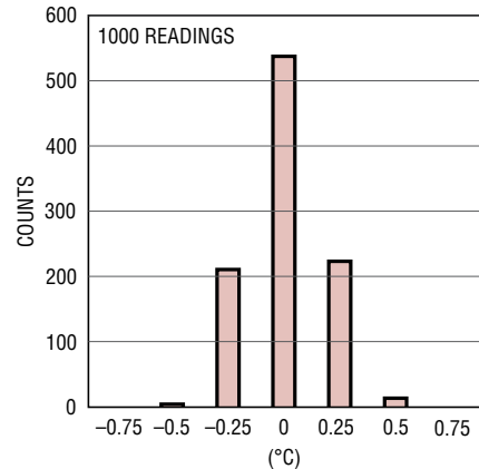
Remote Diode Noise
