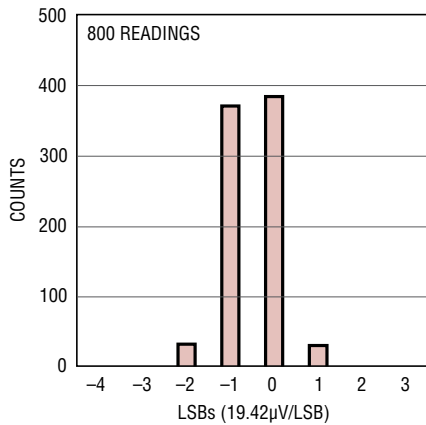
LTC2990 Differential Noise
