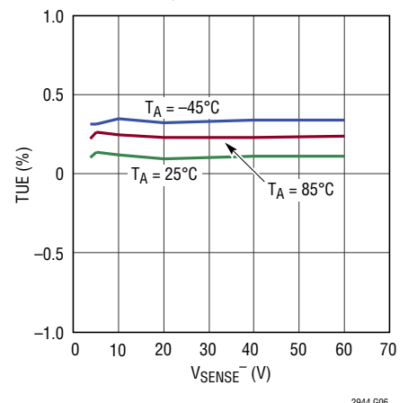
Voltage Measurement ADC Total Unadjusted Error
