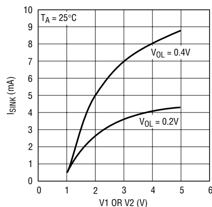
\overline{\text{RST}} , COMPX I_{SINK} vs Supply Voltage
