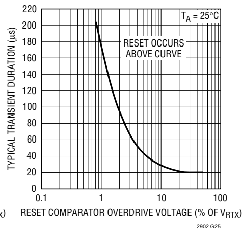
Typical Transient Duration vs Comparator Overdrive (V3, V4)
