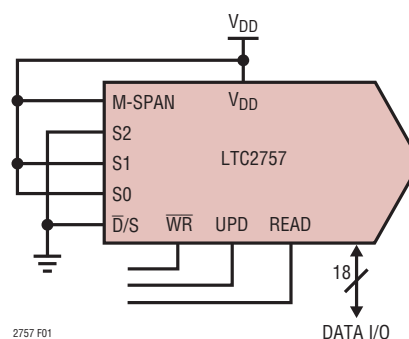
Figure 1. Configuring the LTC2757 for Single-Span Operation (±10V Range)
