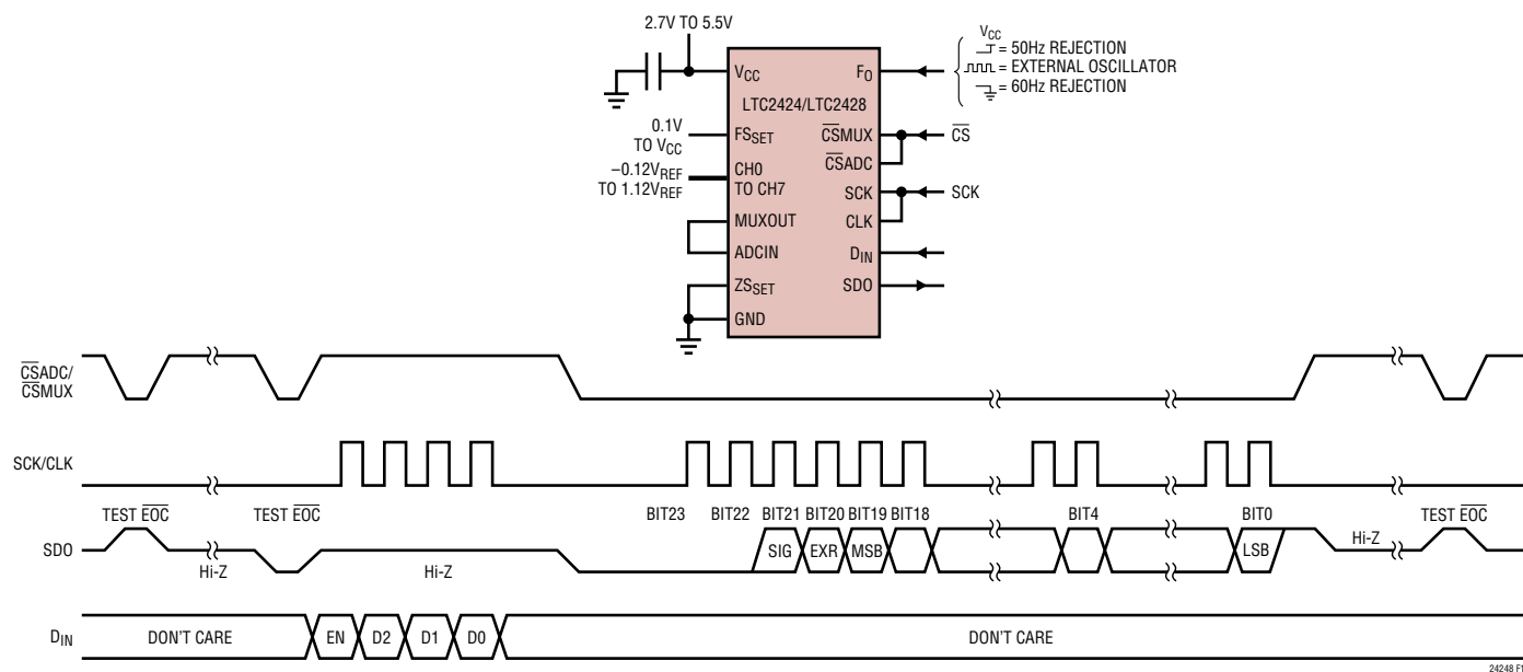
Figure 13. External Serial Clock Timing Diagram
