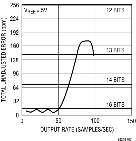
Figure 7. Total Error vs Output Rate (V REF = 5V)
