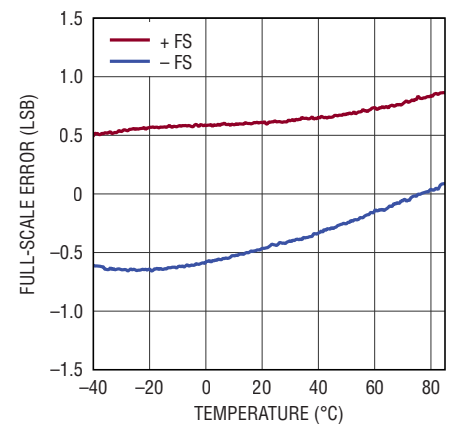
Full-Scale Error vs Temperature, \text{REFBUF} = 4.096\text{V}
