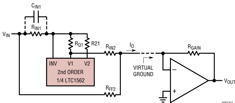
Figure 11. Feedforward Notch Configuration for f_N \geq f_0
