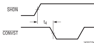
Figure 13a. \overline{\text{SHDN}} to \overline{\text{CONVST}} Wake-Up Timing
