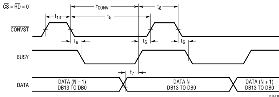
Figure 18. Mode 1b. \overline{\text{CONVST}} Starts a Conversion. Data Outputs Always Enabled ( \overline{\text{CONVST}} = \text{low} )
