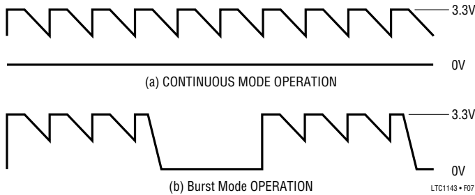
Figure 7. C_T Waveforms
