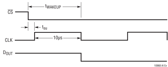
Case 2. Timing Diagram
