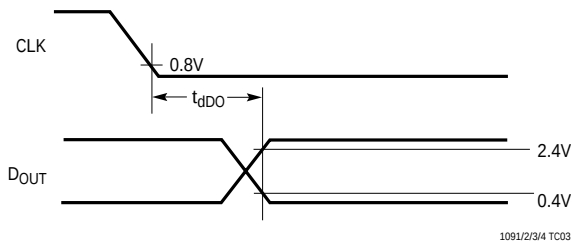
Voltage Waveforms for D_{OUT} Delay Time, t_{dO}
