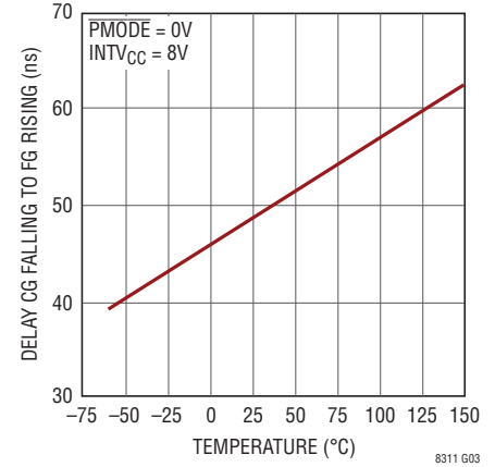
Delay from CG Turn-Off to FG Turn-On
