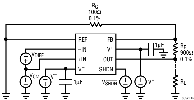
Figure 2. ±5V DC Test Circuit
