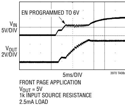
Start-Up from High Impedance Input Source
