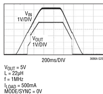
Start-Up Shutdown Waveform I LOAD = 500mA
