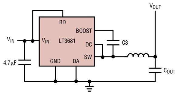
(5c) For V_{OUT} < 2.5V
