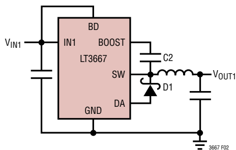
(2b) For V_{OUT1} < 2.2\text{V} ; V_{IN1} < 25\text{V}
