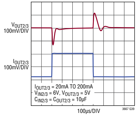
LD0s: Transient Response
