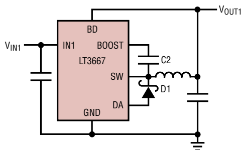
(2a) For V_{OUT1} \geq 2.2\text{V}
