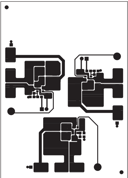
Component Side
