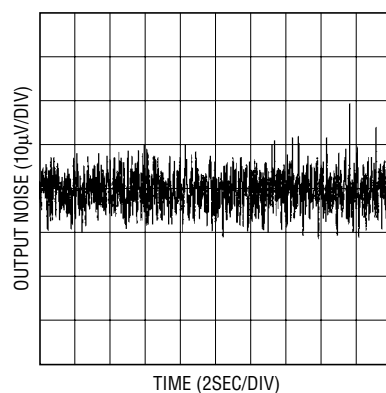
2.5V Output Noise 0.1Hz ≤ f ≤ 10Hz
