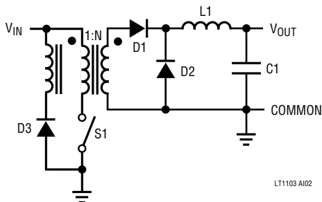
Simplified Forward Converter
