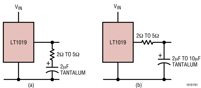
Figure 1. Output Bypassing
