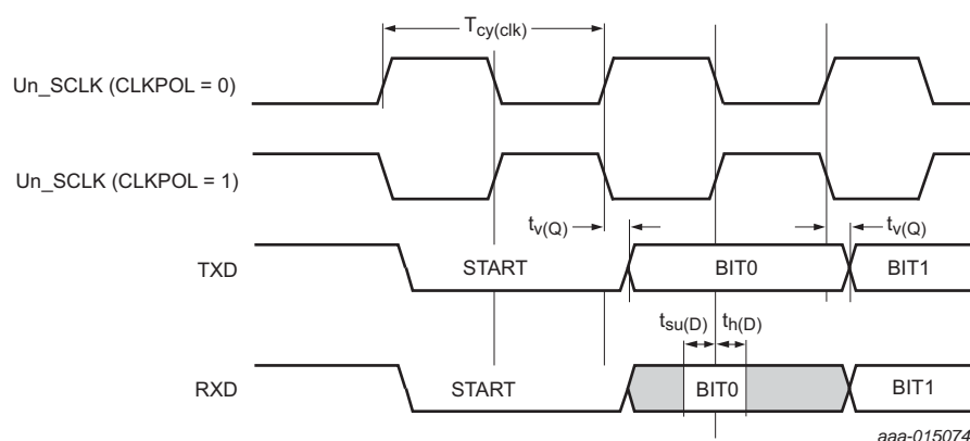
Fig 37. USART timing
