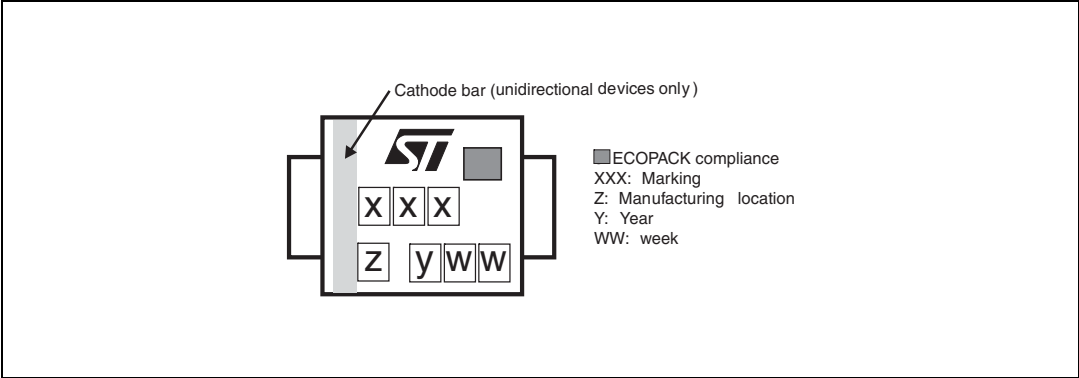
Figure 14. Marking layout
