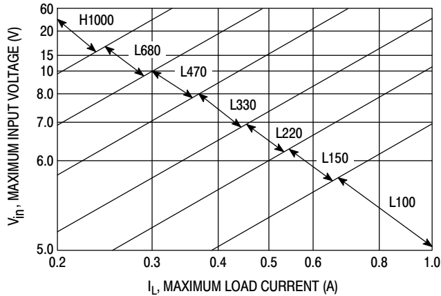
Figure 17. LM2575-3.3
