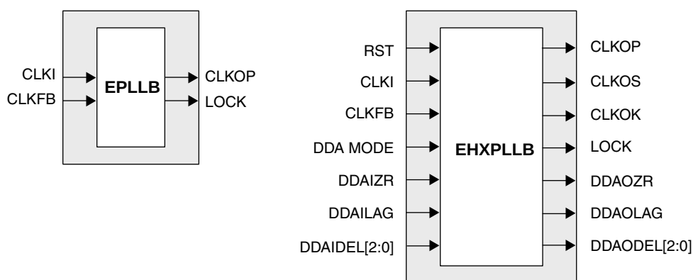
Figure 2-12. PLL Primitive
