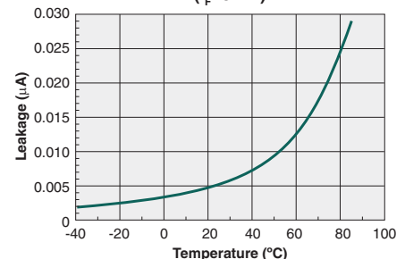
Typical Leakage vs. Temperature Measured Across Pins 4&6 ( I_F = 5\text{mA} )
