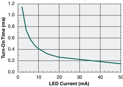
Typical Turn-On Time vs. LED Forward Current
