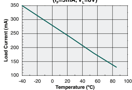
Typical Current Limiting vs. Temperature ( I_F=5\text{mA} , V_L=8\text{V} )
