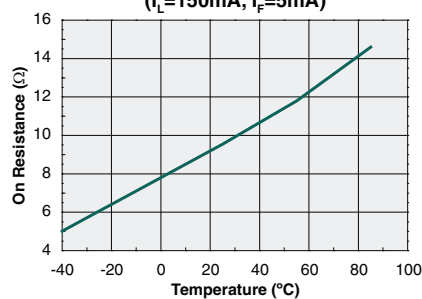
Typical On-Resistance vs. Temperature ( I_L=150\text{mA} , I_F=5\text{mA} )
