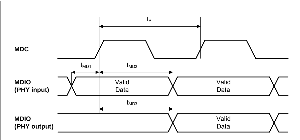
FIGURE 6-3: MDC/MDIO TIMING
