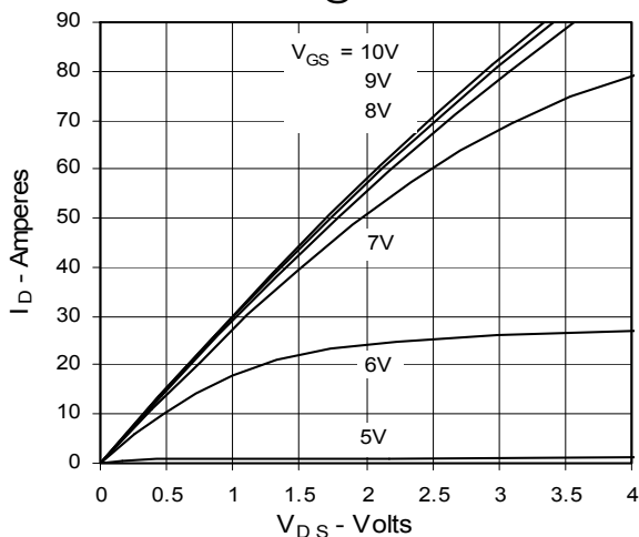
Fig. 1. Output Characteristics @ 25^\circ\text{C}
