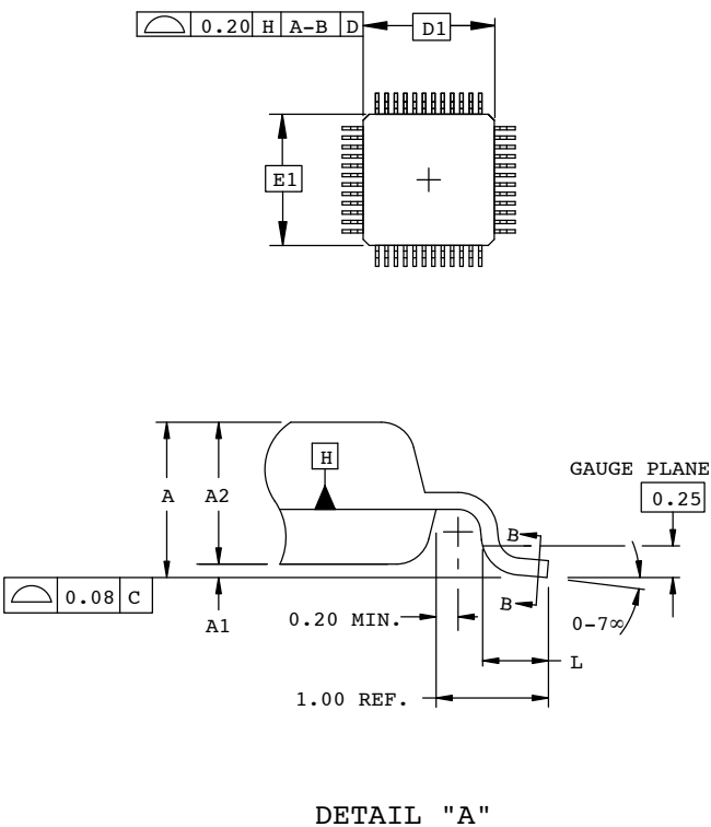
DETAIL "A"
