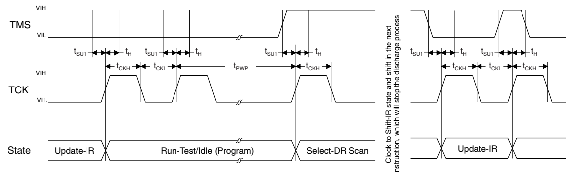
Figure 10. Verify Timing Diagram
