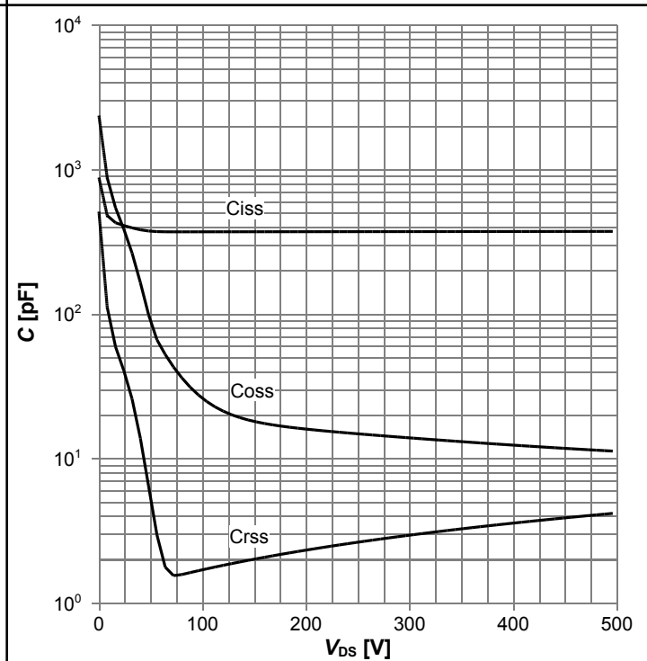
Diagram 18: Typ. capacitances
