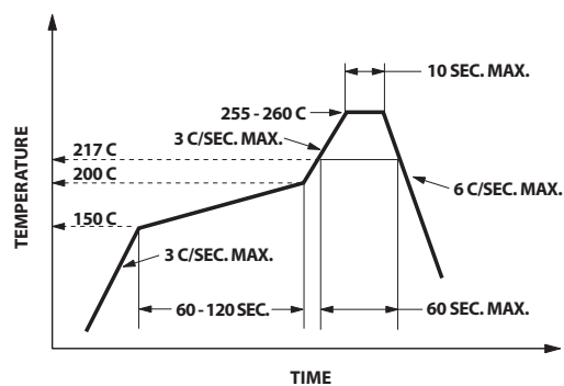
Figure 10. Recommended Pb-free reflow soldering profile.
