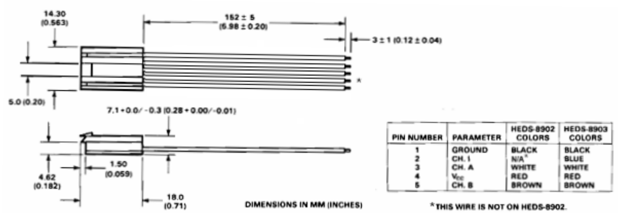
Figure 8. HEDS-8903 Connector.
