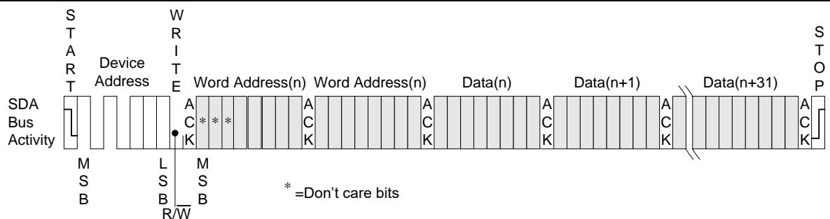
Figure 5-7. Page Write
