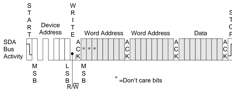
Figure 5-6. Byte Write
