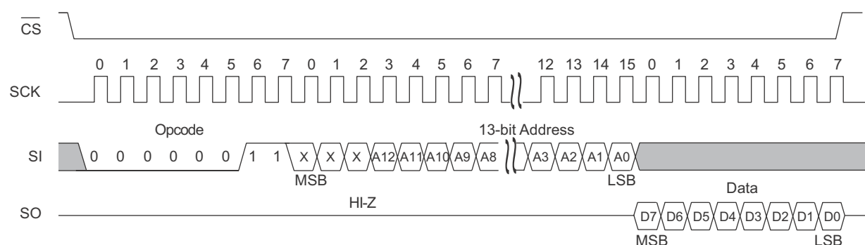
Figure 12. Memory Read
