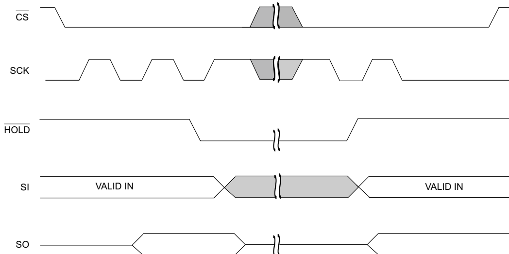
Figure 12. HOLD Operation [2]
