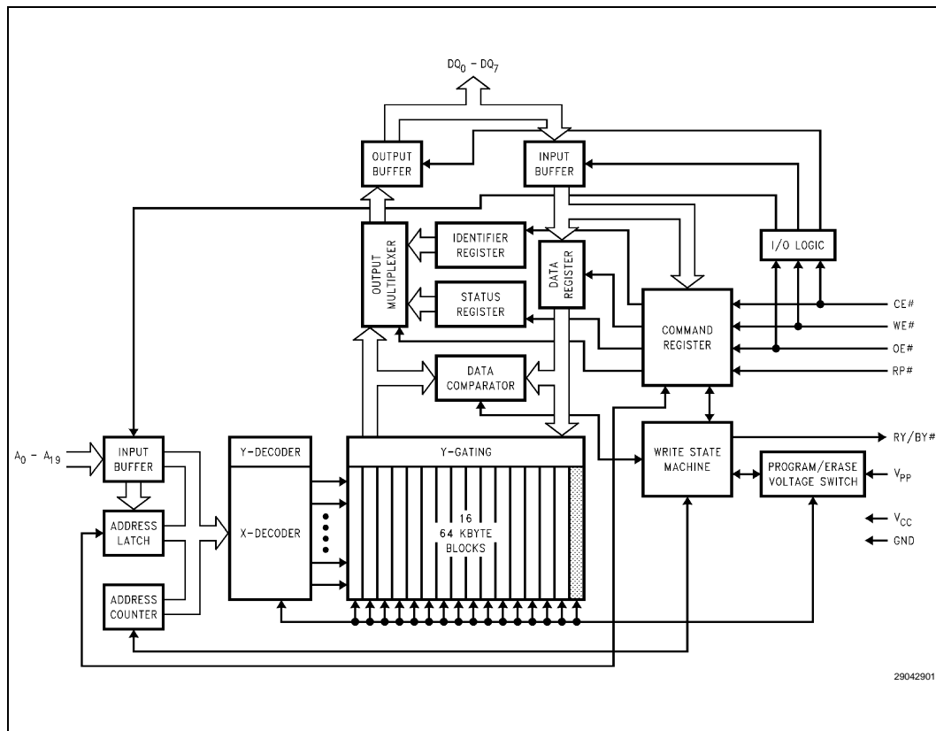
Figure 1. Block Diagram
