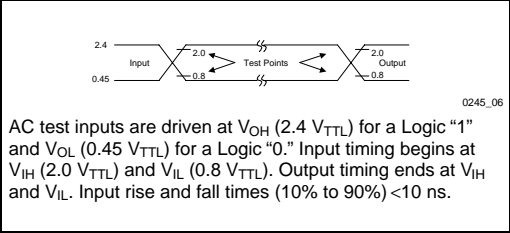
Figure 9. Testing Input/Output Waveform(1)
