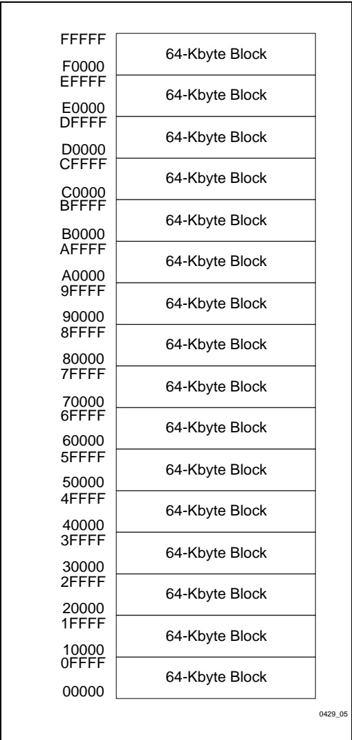
Figure 5. Memory Map
