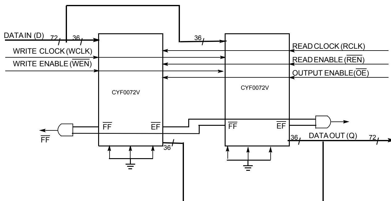
Figure 3. Width Expansion
