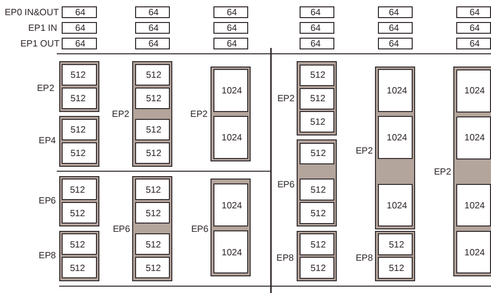
Figure 3-3. Endpoint Configuration
