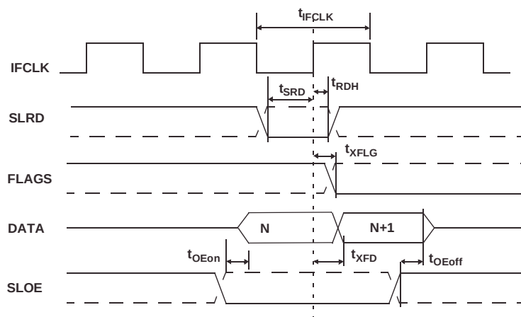
Figure 9-5. Slave FIFO Synchronous Read Timing Diagram [13]
